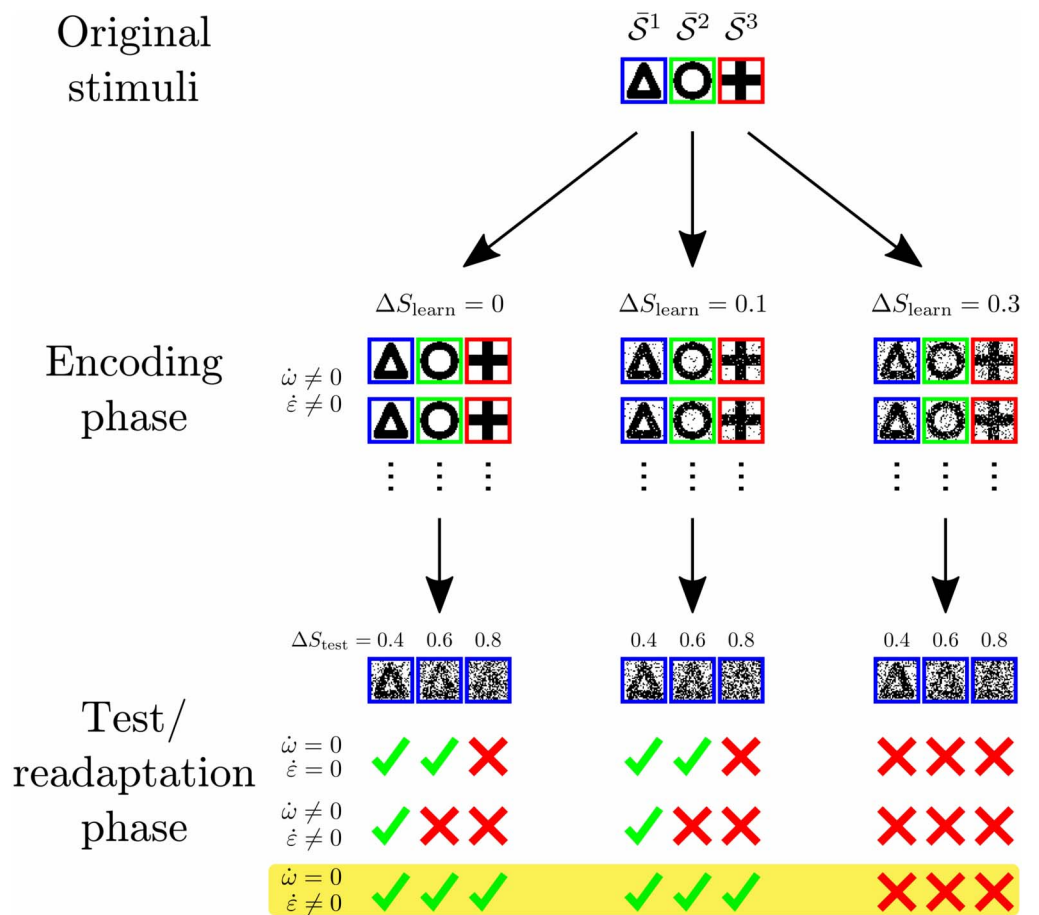
Figure 7. Schematic summary of results. Noisy patterns \mathcal{S}^v are repeatedly generated from original stimuli \bar{\mathcal{S}}^v (e.g., a triangle, a circle, and a cross) and imprinted on the stimulus layer (encoding phase). If the noise \Delta S_{\text{learn}} is sufficiently small, synaptic and intrinsic plasticity lead to the formation of structure encoding the organization of stimuli (existence of different geometrical forms). After this initial learning phase, a second learning or readaptation phase enables the network to classify stimuli even in the presence of very high levels of noise \Delta S_{\text{test}} . Here, only intrinsic plasticity should be present ( \dot{\omega} = 0; \dot{\epsilon} \neq 0 ). This suggests that learning is carried out in two phases: In the first phase, the encoding phase , synaptic weights develop to represent the basic organization of the environmental stimuli. This structuring of synaptic weights is most efficient if the noise \Delta S_{\text{learn}} is low. In the second phase, the readaptation phase , learning is dominated by intrinsic plasticity while synaptic weights have to be maintained. The cortical firing thresholds are then able to quickly adapt to the current level of noise \Delta S_{\text{test}} . Thereby, intrinsic plasticity approximates the optimal thresholds for a given value of \Delta S_{\text{test}} maximizing performance.
