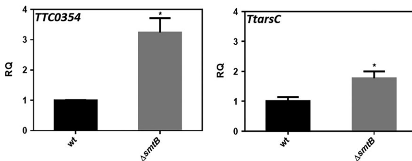
Fig. 6. qRT-PCR analysis of TTC0354 and TtarsC in T. thermophilus HB27 (wt) and \Delta smtB grown without As. The error bars indicate the standard deviation of the average values of two independent experiments in triplicate samples (* P < 0.05 ).
