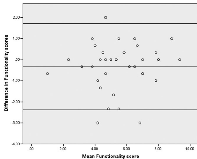
FIGURE 1 Bland and Altman scatterplot for differences in T1-T2 measures of Functionality with 95% limits of agreement
