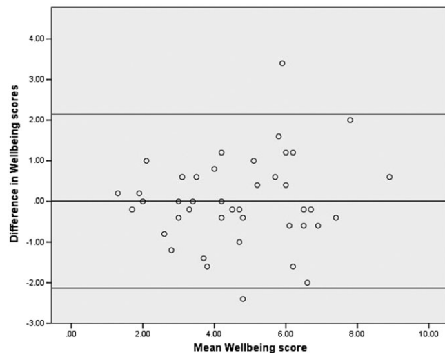
FIGURE 2 Bland and Altman scatterplot for differences in T1-T2 measures of Wellbeing with 95% limits of agreement
