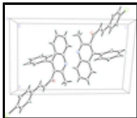
Fig. 2. The molecular packing for C 25 H 18 ClNO viewed down the a axis.
