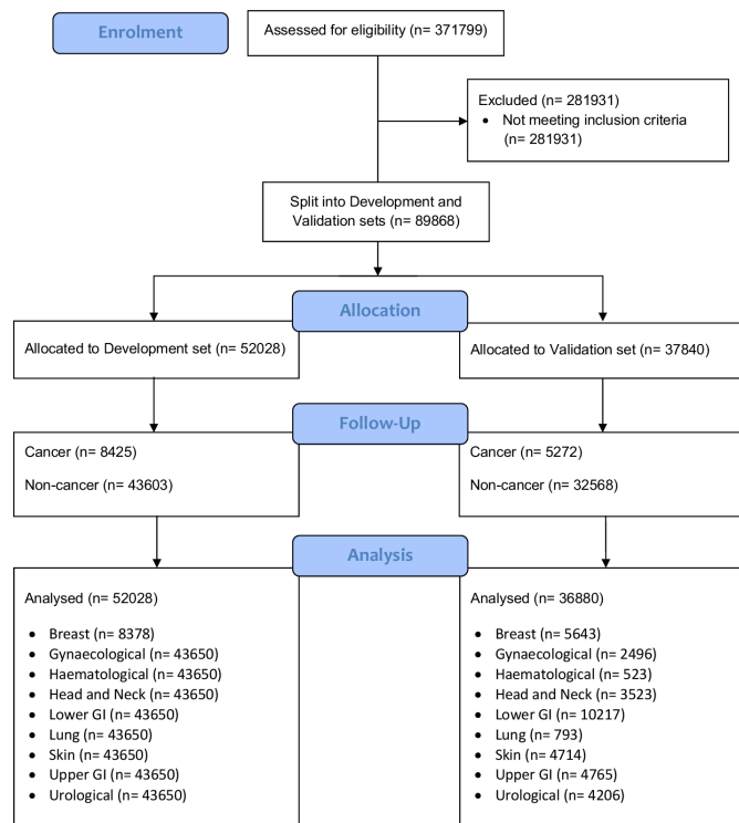
Figure 1 We note that the development set analysed numbers of data points (bottom left) are the same for all pathways with the exception of breast. We discovered during development that modest performance gains could be achieved by using just the 2WW breast pathway data for the breast algorithm, and using the data for all other pathways for each of the other eight algorithms (hence the same training data were used for all pathways except breast). 2WW, 2-week wait. GI, Gastrointestinal.
