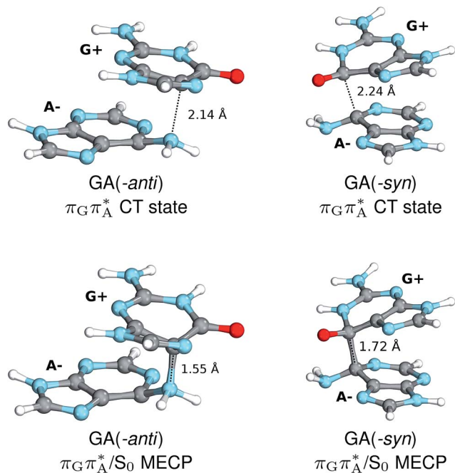
Fig. 5 Geometries of the different G^+A^- S_1 minima located for both GA- syn and - anti conformers (top), and the corresponding S_1/S_0 MECPs (bottom). The optimizations were performed using QM_{\text{bases}}/MM setup, but only the G and A bases are shown for clarity.
