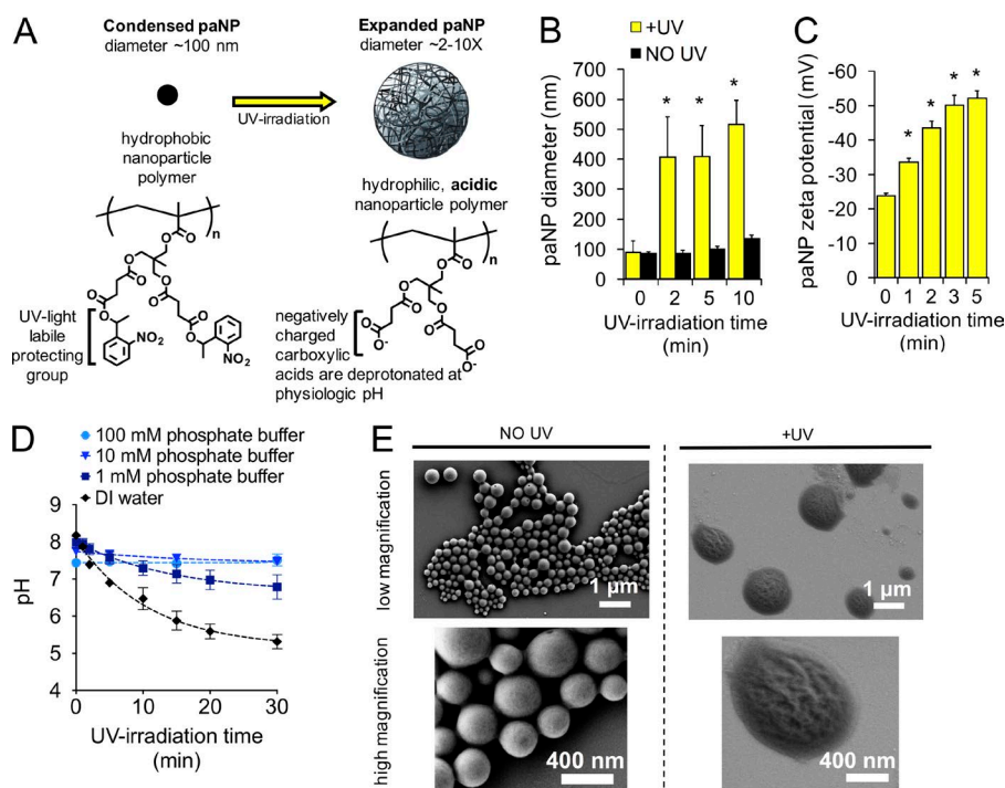
Figure 1. Characterization of UV activation mechanism of paNPs. (A) Schematic of the paNP mechanism of UV-triggered acidification and swelling. (B) Dynamic light scattering characterization measurements of paNP diameter as a function of UV irradiation and duration. paNPs exposed to UV light (yellow bars) increase in diameter by 300–400%; without UV exposure, paNP diameter remains constant ( n = 3 experiments; *, P < 0.05 vs. time 0). (C) Zeta potential (i.e., surface charge) of the paNPs becomes more negative with additional UV irradiation because of the deprotection of additional carboxylic acid functionalities ( n = 3 experiments; *, P < 0.01 vs. time 0). (D) pH of deionized water or pH 7.4 phosphate buffers of increasing buffering strengths (i.e., molarities) as a function of UV irradiation time. (E) Scanning electron micrograph images of paNPs before (left) and after (right) UV irradiation demonstrate UV-triggered swelling. All error data are plotted as mean \pm SD.
