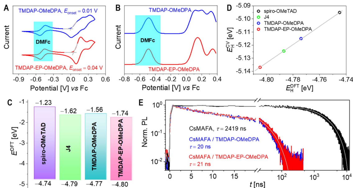
Fig. 2 (A) Cyclic voltammograms with bis(pentamethylcyclopentadienyl)iron (DMFc) as the internal reference. The derived onset potential ( E_{onset} ) of the first oxidation wave is also presented. (B) Square wave voltammograms. (C) The lowest unoccupied molecular orbital energy levels (values above color bars) and the HOMO energy levels ( E_H^{DFT} ) (value under color bars) calculated by the density functional theory method at the B3LYP/6-311G(d,p) level. (D) Correlation between the HOMO energy levels from voltammetric measurement and theoretical calculation. (E) Time-resolved photoluminescence traces of CsMAFA perovskite films with and without an organic semiconductor layer. Note that the broken x-axis was set to be in a partially linear and partially logarithmic mode. The gray lines represent the biexponential fits of normalized photoluminescence intensity as a function of time ( t ), yielding the amplitude-averaged lifetime ( \tau ). The excitation wavelength is 670 nm.
