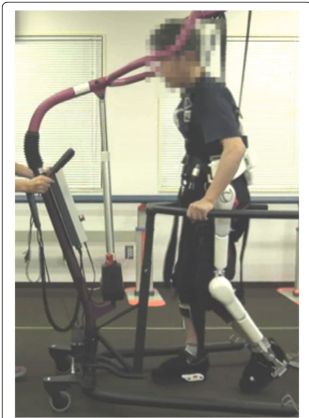
Figure 1 Photograph showing the Hybrid Assistive Limb (HAL) worn by a patient and the All-In-One Walking Trainer suspending the patient during the locomotor training.
