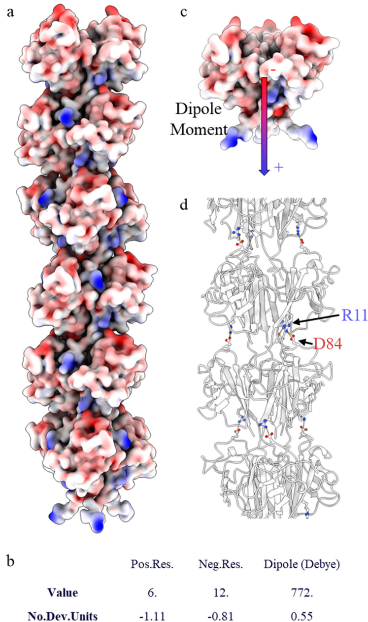
Supporting Figure 4. Surface electrostatics and dipole moment of F-ENA. (a) F-ENA pilus surface colour-coded according to electrostatic potential using ChimeraX; (b) Dipole moment of an F-ENA trimer as calculated by the Protein Dipole Moments Server ( https://dipole.proteopedia.org/ ) and visualized onto a single F-ENA trimer (c); (d) Salt bridges between R11 and D84 that are reinforcing the interaction between two successive F-ENA fiber segments are shown in stick representation.
