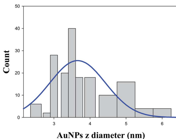
Fig. 6 AFM image for 1.0 \times 10^{-8} M [Au@tiopronin] in the presence of [\text{Ru}(\text{bpy})_3]^{2+} and corresponding histogram from which the average diameter obtained was 3.7 \pm 0.6 nm.
