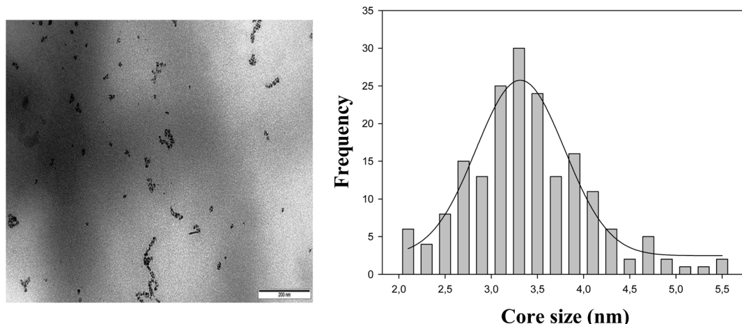
Fig. 2 TEM image (left) and size distribution (right) of the tiopronin gold nanoparticles in the absence of the Ru(II) complex and presence of the cacodylate buffer at pH 7.0.
