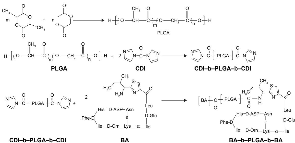
Figure 1 Schematic illustration of the synthetic steps of BA-b-PLGA-b-BA. Abbreviation: BA, bacitracin A.
