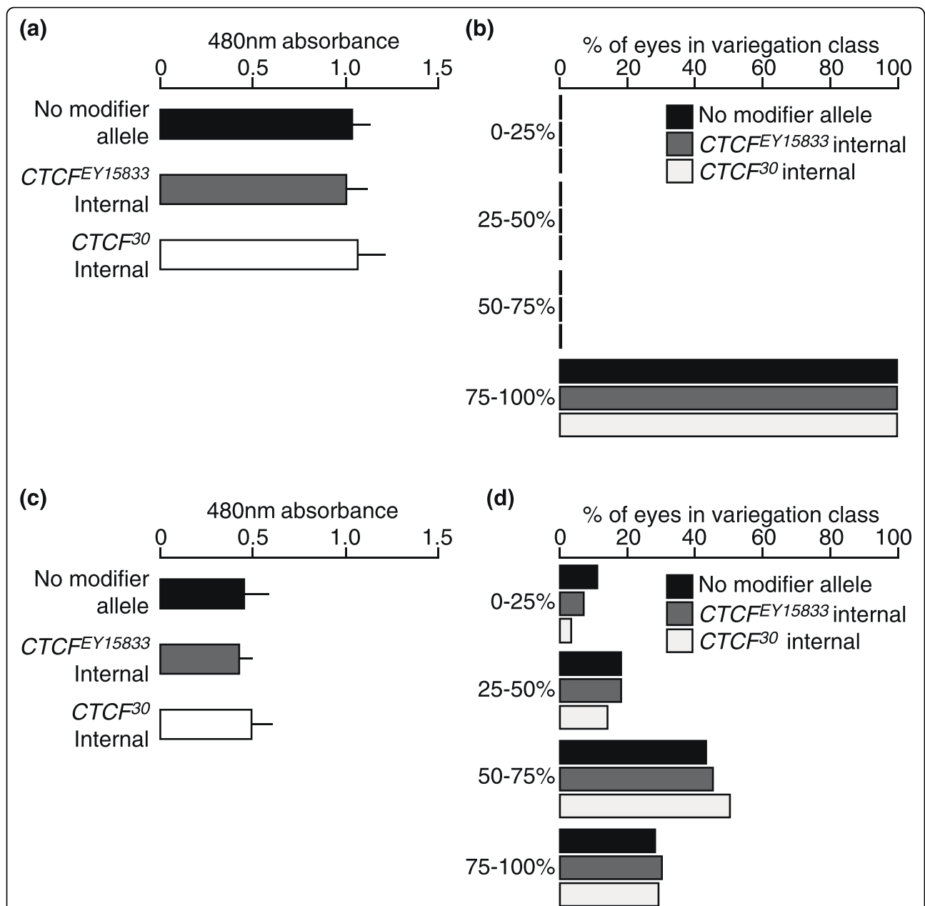
Figure 3 Absence of maternal or paternal effects from mutant dCTCF on Dp(1;f)LJ9 garnet expression. External control progeny (no modifier allele) have the same genotype as internal control progeny ( y 1 z 2 g 53d /Dp(1;f)LJ9; TM3, Sb Ser/+ ) but are generated from a separate cross with parents that have never encountered a mutant CTCF X allele. (a) Maternally inherited Dp(1;f)LJ9 CTCF X internal control eye pigment levels; no significant difference in pigment levels was observed between external control progeny (no modifier allele) and internal control progeny from fathers carrying CTCF X ( CTCF X internal), demonstrating that no paternal effect occurs. (b) Phenotypes of maternally inherited Dp(1;f)LJ9 ranging from 0% to 100% pigmentation; No modifier allele n = 300, CTCF EY15833 internal n = 300, CTCF 30 internal n = 300. No garnet variegation was detected from the internal controls. (c) Paternally inherited Dp(1;f)LJ9 CTCF internal control eye pigment levels; no significant difference in pigment levels was observed between the external control progeny (no modifier allele) and internal control progeny from mothers carrying CTCF X ( CTCF X internal), demonstrating that no maternal effect occurs. (d) Phenotypes of paternally inherited Dp(1;f)LJ9 ranging from 0% to 100% pigmentation; no modifier allele n = 300, CTCF EY15833 internal n = 300, CTCF 30 internal n = 300. No significant change in garnet variegation was detected from the internal controls. Red eye pigment levels are measured by absorbance at 480 nm, and pigment quantification mean values for each group are based on n = 5 samples (40 heads total); error bars represent standard deviation.
