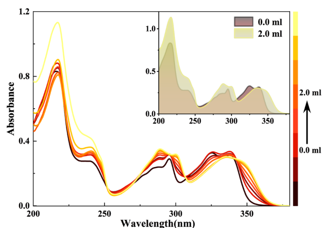
Fig. 5 UV-Vis spectra of a 2.5 \times 10^{-5} \text{ M} HBI-pBr solution in \text{CH}_3\text{OH} as a function of \text{CF}_3\text{COOH} (TFA, 2.0 \times 10^{-4} \text{ M} ) in \text{CH}_3\text{OH} from 0 to 2.00 mL.
