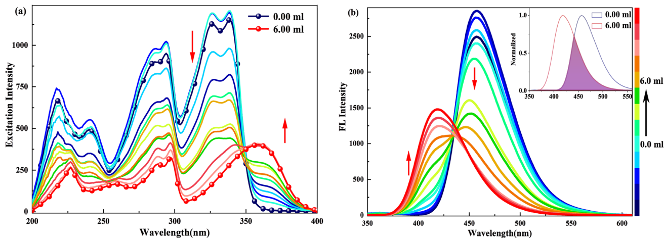
Fig. 4 (a) Excitation ( \lambda_{\text{em}} = 419.0 \text{ nm} ) and (b) emission spectra ( \lambda_{\text{ex}} = 340.0 \text{ nm} ) of 2.5 \times 10^{-5} \text{ M} HBI-pBr in \text{CH}_3\text{OH} as a function of 2.0 \times 10^{-4} \text{ M} [(\text{Bu})_4\text{N}]\text{OH} solution in \text{CH}_3\text{OH} from 0 to 6.00 mL.
