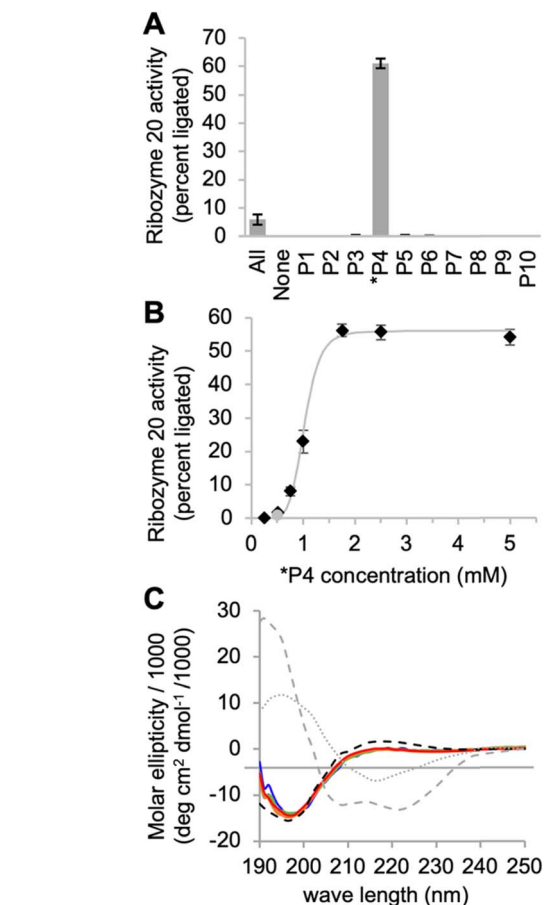
Fig. 4 Interactions of ribozyme 20 with individual peptides. (A) Activity of ribozyme 20 in the presence of ten individual peptides, each at 5 mM, while the reaction with all peptides ('All') contains each peptide at 0.5 mM concentration. Error bars are standard deviations from three experiments. (B) Titration of peptide 4 into the activity assay of ribozyme 20. The grey line serves to illustrate the saturation at 1.75 mM peptide. The grey data point stems from the presence of all peptides, each at 0.5 mM. Error bars are standard deviations from three experiments. The grey line is a double exponential curve fit to illustrate the sigmoidal behavior. (C) CD spectra of peptide *P4 under the same ion conditions as the ribozyme reactions above. The peptide was tested at four different concentrations (blue: 0.5 mM; green: 1 mM; orange: 1.5 mM; red: 2 mM). The ideal CD spectra of possible peptide secondary structures 43 are shown for alpha helix (grey, dashed), beta sheet (grey, dotted) and random coil (black, dashed).
