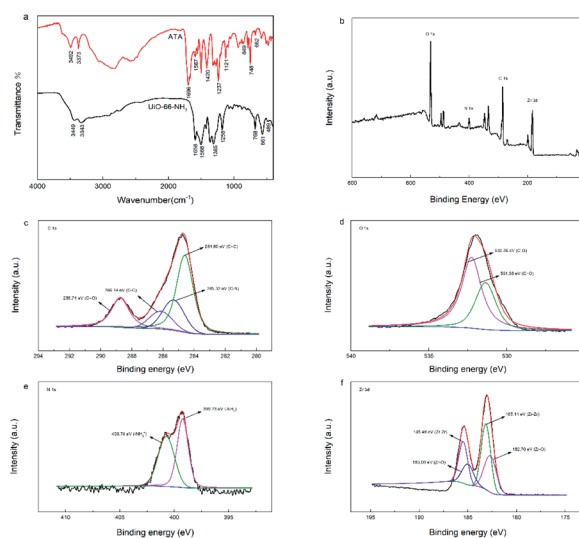
Fig. 3 FT-IR spectra of ATA, and UiO-66-NH 2 (a), and XPS spectra of survey (b), C 1s (c), O 1s (d), N 1s (e) and Zr 3d (f) for the UiO-66-NH 2 .
