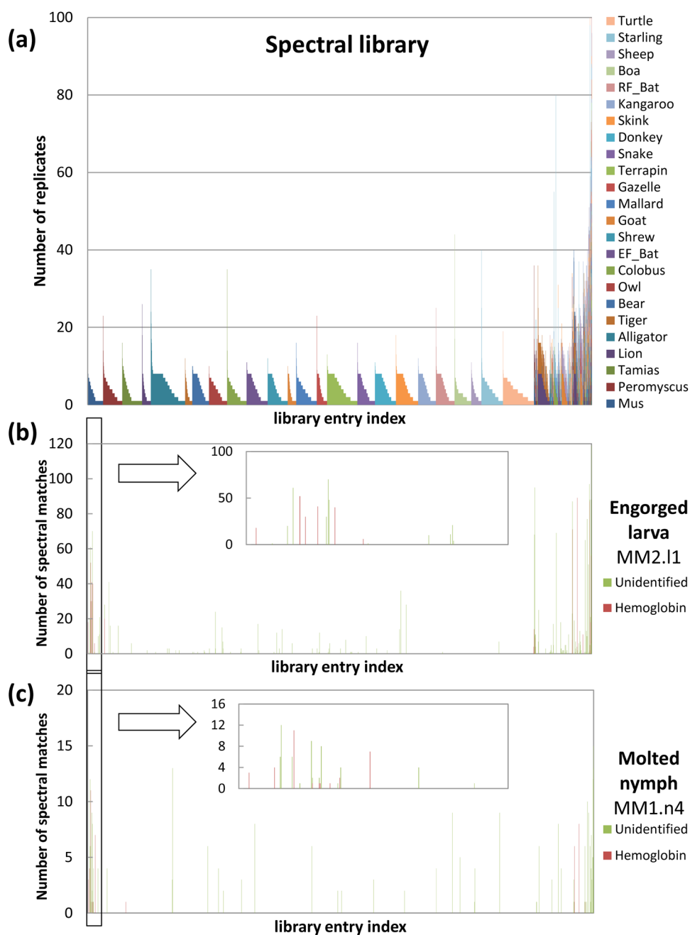
Figure 2. Reference spectral libraries of the blood proteomes of 24 vertebrate species (a) The diversity and abundance of unique and shared spectra in the spectral reference libraries visualized as a bar chart. Each bar along the abscissa represents a distinct consensus spectrum and the height of the bar represents the number of replicates merged into that consensus. Bars are color-coded to represent the species from which the replicates originate. The multi-colored bars to the right represent spectra that are observed in multiple species. Example of spectral dataset matches for (b) one larva engorged with M. musculus (MM2.11), or (c) one molted nymph held at 25 °C for 6 months after feeding on M. musculus (MM1.n4). The majority of spectral matches for the tick datasets are to library spectra from
