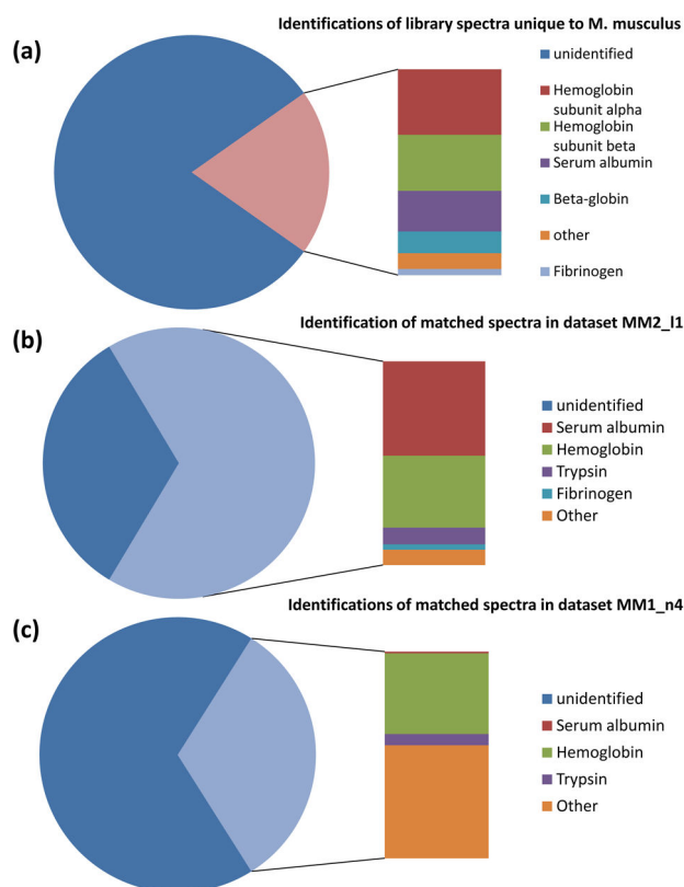
Figure 3. Underlying protein distribution of the blood proteome of M. musculus Peptide identifications of spectra used to build or search the M. musculus library by sequence searching. (a) The protein distribution of the identifications of the library spectra unique to M. musculus . (b & c) the protein distributions of identifications of spectra matched to the M. musculus library for two datasets: MM1.n4 (a molted nymphal tick) and MM2.11 (an engorged larva), respectively. A large fraction of spectra remain unidentified by sequence searching, despite the comprehensiveness of the M. musculus protein sequence database. Among identified spectra, subunits \alpha and \beta of hemoglobin, serum albumin, \beta -globin, and fibrinogen are the most frequent protein identifications found.
