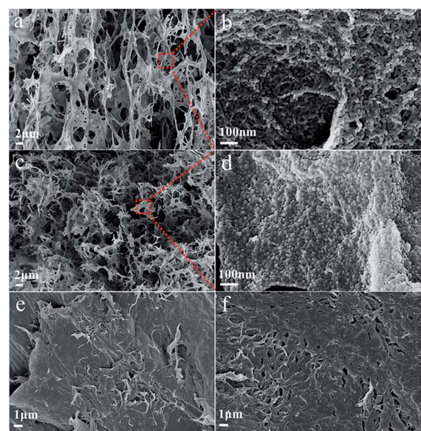
Fig. 3 Structural characterization of chitin-derived carbons: the SEM images of CNC-800 (a and b), CNC-900 (c and d), chitin-800 (e), chitin-900 (f).
