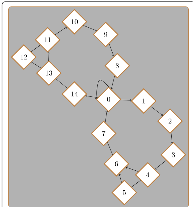
Figure 3 HMM state transitions. An example of a typical HMM state transition diagram. This HMM jointly models background sequence and binding sites from a gapped PWM of length 7. State 0 is the background state. The two arms leading out from state 0 generate binding sites on the positive and negative strands. States 1 and 14 are the first states for binding sites generated in the positive and negative direction respectively. Similarly states 5 and 12 represent the optional base for binding sites generated in the positive and negative direction respectively. When training the HMM various parameters are tied so that they are always equal. For example, the transition parameter from state 0 to state 1 is tied to the parameter for the equivalent transition to state 14. This ensures binding sites are equally likely on both strands of DNA. Similarly emission parameters are tied to ensure binding sites on the negative strand have a distribution that is the reverse complement of the distribution of the binding sites on the positive strand.
