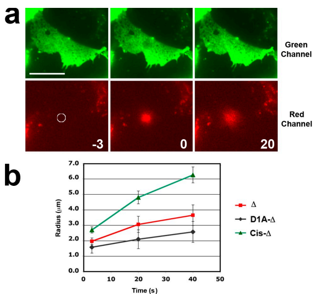
Figure 2. Dendra diffusion assay with cells expressing EcDn \Delta , D1A-EcDn \Delta , and Cis-EcDn \Delta . (a) The circular areas (diameter = 2.5 \mu\text{m} ) in the selected cell–cell contact of EcDn \Delta cells, which express relatively high level of the mutants ( -3 ), was photoconverted from green to red fluorescence (the photoconverted area is circled in the red channel image). The region was imaged at 3 and 23 s (0 and 20) after photoconversion in both green and red channels. Image acquisition time was 1 s. Bar, 10 \mu\text{m} . (b) The experiment shown in panel a was repeated 10 times with each of the indicated cell lines. Error bars indicate SDs. The graph shows the expansion of the red fluorescence area.
