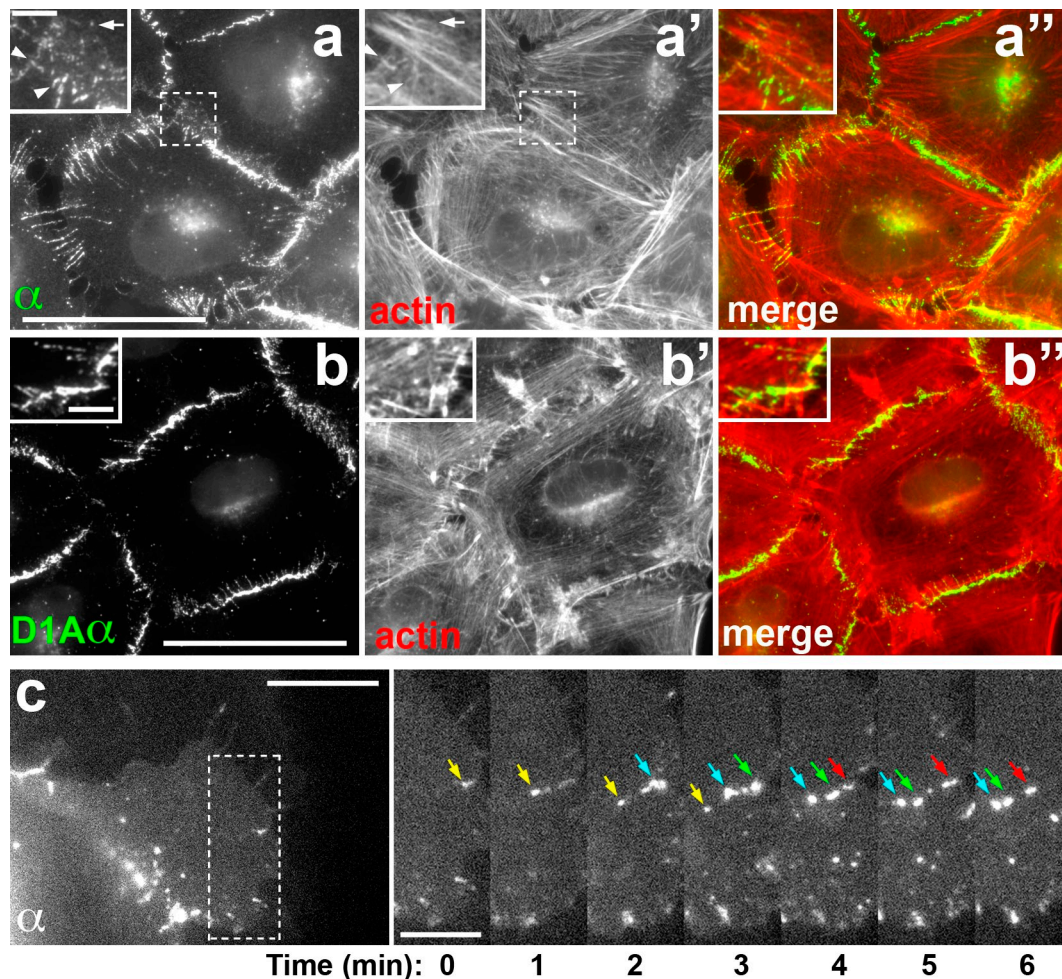
Figure 3. Distribution and dynamics of the EcDn \Delta - \alpha ABD clusters. (a–b'') Double-label immunofluorescence microscopy of A431D cells expressing EcDn \Delta - \alpha ABD (a, \alpha ) or D1A-EcDn \Delta - \alpha ABD (b, D1A \alpha ) chimeras. Cells were stained for chimeras using the anticadherin antibody (a and b) and for F-actin using Alexa Fluor 555 phalloidin (a' and b', actin). The corresponding images are merged in a'' and b''. Note that most of the cadherin clusters (two of the subapical and one of the basal clusters are indicated by arrowheads and an arrow in the insets) associated with actin bundles (Fig. 3 a'). Bars: (main images) 40 \mu m; (insets) 5 \mu m. (c) Time-lapse series (right) of EcDn \Delta - \alpha ABD clusters (frames are indicated according to Video 3 ) present in the boxed region of the left image. Arrows of the same color indicate the same clusters in consequent frames. Note that the clusters produced by this chimera had a much longer lifetime than the tailless clusters and exhibited directional movements. Bars: (left) 10 \mu m; (right) 5 \mu m.
