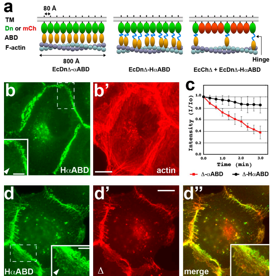
Figure 9. A hinge between Dendra and \alpha ABD changes properties of the clusters. (a) The models of cadherin clusters made from EcDn \Delta - \alpha ABD (EcDn \Delta - \alpha ABD), from hinge-containing EcDn \Delta -H \alpha ABD (EcDn \Delta -H \alpha ABD), and from a combination of EcDn \Delta -H \alpha ABD and the tailless mutant EcCh \Delta (EcDn \Delta -H \alpha ABD + EcCh \Delta ). Note that the hinge (blue) connecting the Dendra2 tag (Dn) and \alpha ABD (yellow) allows connection of each cadherin molecule in the cluster with F-actin. Such clusters could be very stable. In contrast, the lack of the hinge hampers interactions of the majority of cluster molecules with F-actin, resulting in cluster instability. ABD, actin-binding domain; TM, transmembrane domain; mCh, mCherry. (b and b') Immunostaining of EcDn \Delta -H \alpha ABD-expressing cells for the chimera (b, H \alpha ABD) and for actin filaments (b', actin). Note that the apical cell-cell contact areas exhibit no filopodia-like protrusions, and the lateral areas (arrowhead) have no lateral clusters. (c) Dendra photoconversion assay of the clusters in cells expressing EcDn \Delta - \alpha ABD ( \Delta - \alpha ABD) and EcDn \Delta -H \alpha ABD ( \Delta -H \alpha ABD). See Fig. 7 c for other details. Note that the hinge significantly stabilized the clusters. The error bars represent SD (n = 30). (d-d'') A431D cells coexpressing EcDn \Delta -H \alpha ABD (d, green, H \alpha ABD) and EcCh \Delta (d', red, \Delta ). Both images are merged in d''. Note that, upon coexpression with the tailless cadherin mutant, the hinge-containing EcDn \Delta -H \alpha ABD produced many lateral clusters (arrowhead) and resulted in formation of numerous filopodia on the subapical area of cell-cell contact regions. Bars: (main images) 10 \mu m; (insets) 3 \mu m.
