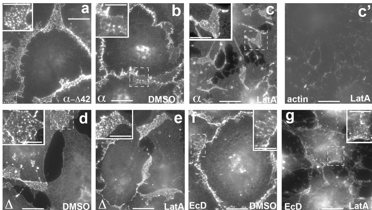
Figure 5. Cluster stability depends on the actin cytoskeleton. (a) Immunolocalization of the EcDn \Delta - \alpha ABD- \Delta 42 chimera ( \Delta 42). Note that the 42- \alpha -long terminal deletion of the \alpha ABD that inactivates binding of this domain to F-actin abolished apical concentration of the clusters and resulted in formation of numerous small clusters typical for EcDn \Delta . Bar, 10 \mu m. (b–g) Effect of actin depolymerization on cadherin clustering during low to high calcium switch: Cells expressing EcDn \Delta - \alpha ABD chimera (b and c; \alpha ), tailless EcDn \Delta chimera (d and e; \Delta ), and full-size Dendra-tagged E-cadherin (f and g; EcD) were cultured at low calcium and then moved to high calcium media in control conditions (b, d, and f; DMSO) or in presence of 8 \mu M of latrunculin A (c, e, and g; LatA). Cells were fixed 5 min after the calcium switch and immunostained for cadherin and the actin cytoskeleton (actin, shown only in c'). The boxed areas are enlarged in the insets. Magnifications are the same in all images. Note that depolymerization of F-actin by latrunculin A prevented concentration of the EcDn \Delta - \alpha ABD clusters along the apical area of cell–cell contacts and significantly inhibited formation of the EcDn junctions but has little effect on clustering of the tailless EcDn \Delta cadherin. Bars: (main images) 10 \mu m; (insets) 5 \mu m.
