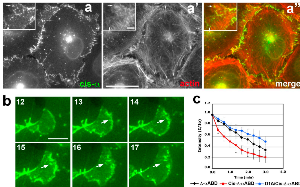
Figure 7. \alpha ABD cooperates with the cadherin cis-interface. (a–a'') Immunostaining for the cis-EcDn \Delta - \alpha ABD chimera (a) and for actin filaments (a'). Note that many cadherin clusters were still associated with the actin filaments (some are indicated by the arrows) and concentrated along the apical region of the cell–cell contacts. Bars: (main images) 20 \mu m; (insets) 2.5 \mu m. (b) Time-lapse imaging of the cis-EcDn \Delta - \alpha ABD clusters (frames are indicated according to Video 6). The movement of one of the clusters is traced by the arrows. Note that the clusters are stable and exhibit basal to apical movement. Bar, 5 \mu m. (c) Dendra photoconversion assay of the clusters in cells expressing EcDn \Delta - \alpha ABD ( \Delta - \alpha ABD), cis-EcDn \Delta - \alpha ABD (Cis- \Delta - \alpha ABD), and D1A/Cis-EcDn \Delta - \alpha ABD (D1A/Cis- \Delta - \alpha ABD). The graph shows changes in intensity of the red fluorescence in the individual junctions over time (in minutes) after the Dendra2 green to red photoconversion. The error bars represent SD ( n = 30 ).
