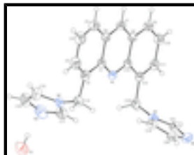
Fig. 1. The structure of the title compound, showing the atom-numbering scheme and intramolecular hydrogen bond. Displacement ellipsoids are drawn at the 30% probability level.
