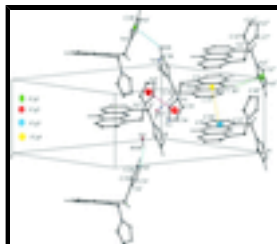
Fig. 2. C–H...O, O–H...N, C–H... \pi and \pi — \pi interactions (dotted lines) in the title compound. Cg denotes ring centroid. [Symmetry code: (i) -1/2 - x, 1/2 + y, 1/2 - z ; (ii) -x, 1 - y, -z ; (iii) 1 - x, 2 - y, -z ; (iv) 1 - x, 1 - y, -z ; (v) 1/2 - x, 2 - y, -z ]
