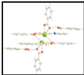
Fig. 2. The dimer structure of complexes, formed by the weak intermolecular Pb...O interactions (dashed lines in violet).
