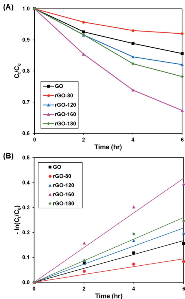
Fig. 6 (A) Photocatalytic degradation of MB dye normalized against adsorption, (B) pseudo-first order kinetic plot of MB dye, in the presence of GO, rGO-80, rGO-120, rGO-160 and rGO-180.
