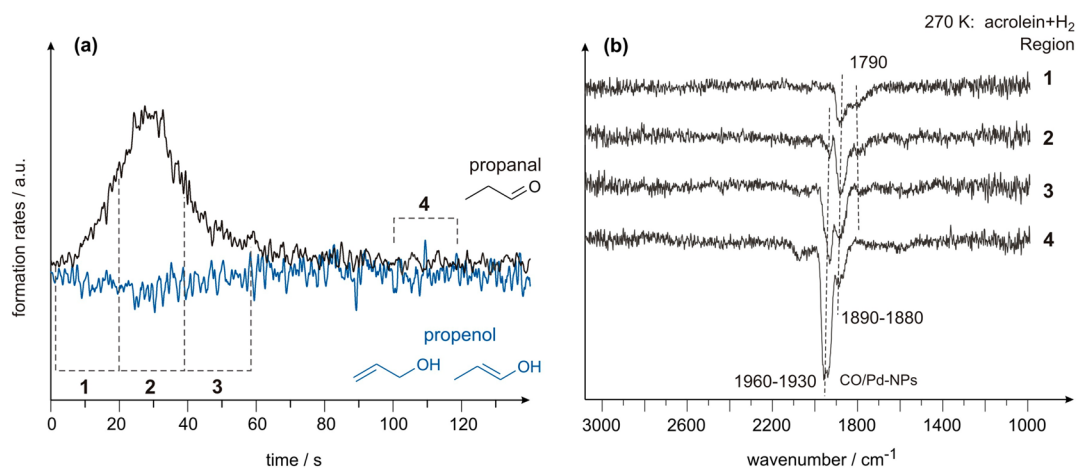
Figure 4. (a) Formation rate of propenol (blue line) and propanal (black line) on 12 nm sized supported Pd nanoparticles at 270 K under continuous exposure of \text{H}_2 and acrolein. (b) IR spectra obtained on Pd nanoparticles turning over. Spectra 1–4 correspond to the regions 1–4 indicated in (a).
