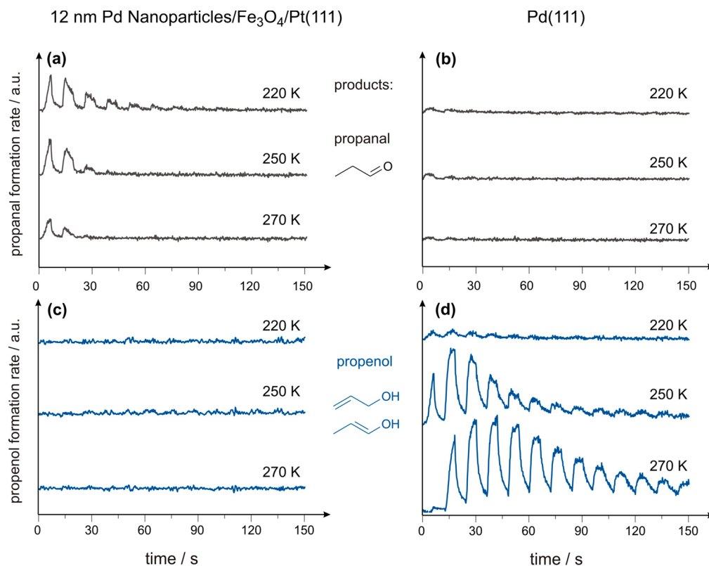
Figure 1. Formation rates of the reaction products—propanal (upper row) and propenol (lower row)—on 12 nm sized supported Pd nanoparticle (a, c) and Pd(111) (b, d) during continuous dosing of H 2 and pulsed dosing of acrolein at different temperatures.
