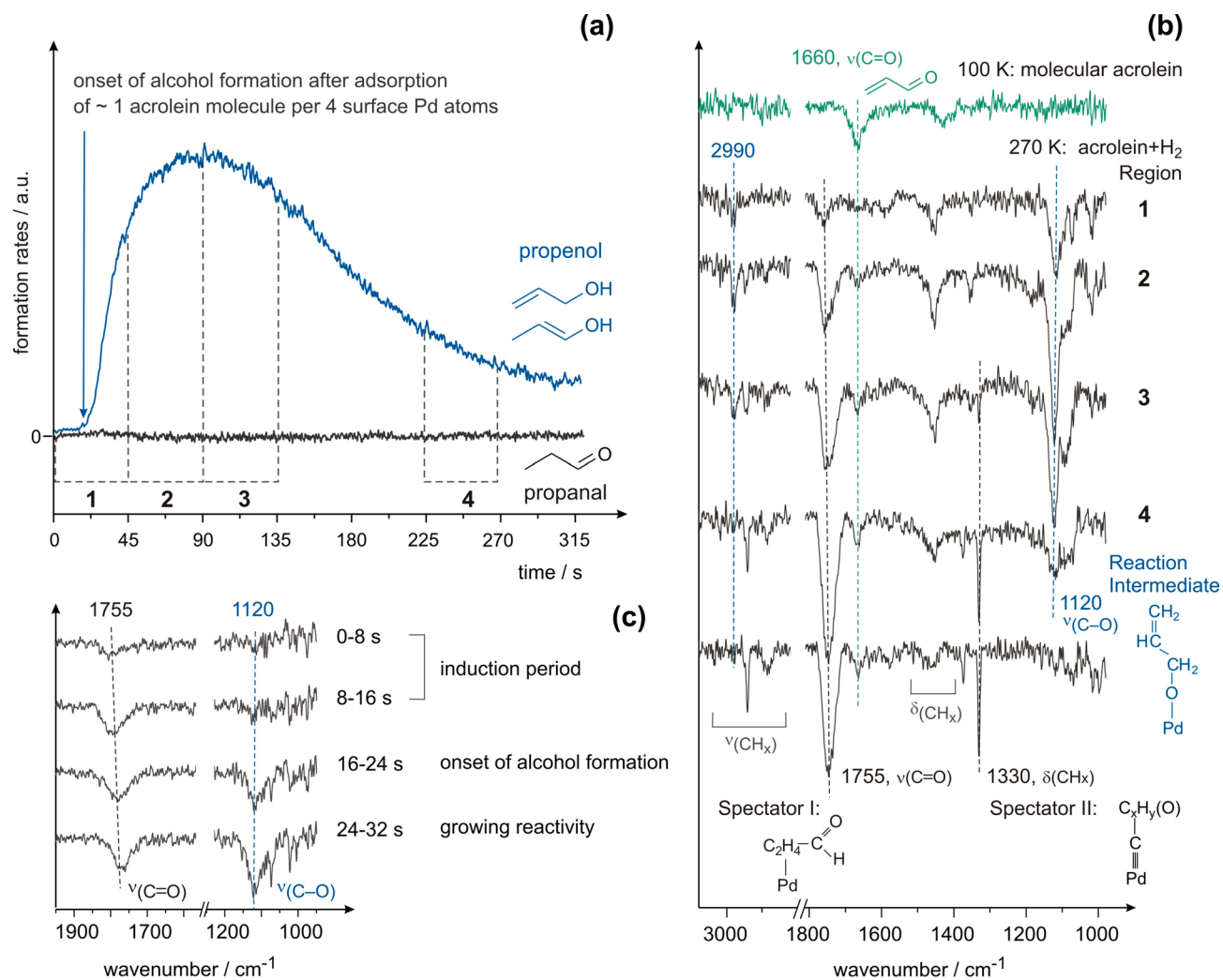
Figure 2. (a) Formation rate of propenol (blue line) and propanal (black line) on Pd(111) at 270 K under continuous exposure of \text{H}_2 and acrolein. (b) IR spectra obtained for a monolayer of molecularly adsorbed acrolein at 100 K on pristine Pd(111) (green line) and on Pd surface turning over at 270 K during a continuous exposure to acrolein and \text{H}_2 . Spectra 1–4 correspond to the regions 1–4 indicated in (a). The lowest spectrum is obtained after 450 s of acrolein exposure after the propenol formation rate has dropped to zero. (c) IR spectra obtained on Pd(111) surface turning over with higher time resolution during the induction period and period of growing reactivity.
