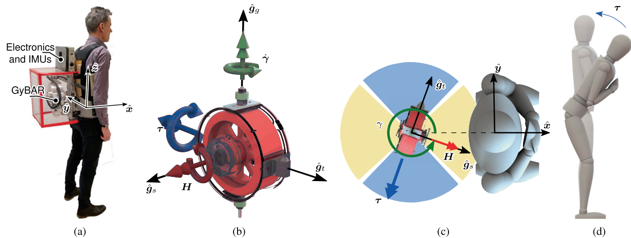
Figure 1. GyBAR prototype wearable gyroscopic actuator. (a) Model wearing the prototype GyBAR used in the experiments. (b) Simplified gyroscopic moment, \tau \approx -\tau\hat{g}_t , is proportional to the angular momentum, H = H\hat{g}_s , of a spinning mass and the angular rate, \dot{\gamma} = \dot{\gamma}\hat{g}_g , at which the motorized frame is gimbaled (Eq. 2). (c) The GyBAR-fixed coordinate frame (\hat{g}_x, \hat{g}_y, \hat{g}_z) is initially aligned with the human-fixed frame (\hat{x}, \hat{y}, \hat{z}) prior to rotation by the gimbal angle, \gamma , about the axis \hat{g}_z \parallel \hat{z} . This angle is controlled to orient \tau in the direction of interest: the blue region for assistance in the sagittal plane, or the yellow region for assistance in the frontal plane. (d) Example use of a moment to restore upright posture in the sagittal plane.
