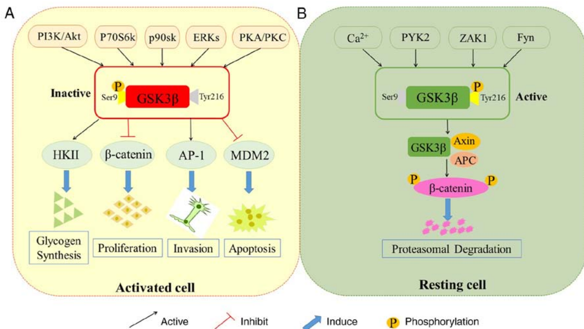
Figure 2. Regulatory mechanisms of GSK 3β. The activity of GSK 3β can be inactivated by multiple pathways. PI3K/Akt, P70S6k, p90sk, ERKs and PKA/PKC can attenuate GSK 3β enzymatic activity by phosphorylating GSK 3β at Ser9. Inhibition of GSK 3β activity leads to the stabilization and accumulation of β-catenin in the cytosol. GSK 3β inactivation is also involved in glycogen synthesis, protein synthesis, cell proliferation and cell invasion. Additionally, PYK2, Ca 2+ , ZAK1 and Fyn are able to phosphorylate GSK 3β at Tyr216, which increases the GSK 3β activity. Subsequently, activated GSK 3β phosphorylates downstream target β-catenin. GSK 3β, glycogen synthase kinase3β; PI3K, phosphoinositide3 kinase; P70S6K, P70S6 kinase; ERKs, extracellular signal-regulated kinases; PKC, protein kinase C; PKA, protein kinase A; HKII, hexokinase II; AP-1, activating protein-1; MDM2, murine double minute 2; PYK2, proline-rich tyrosine kinase 2; ZAK1, Zaphod kinase 1; APC, adenomatous polyposis coli.
