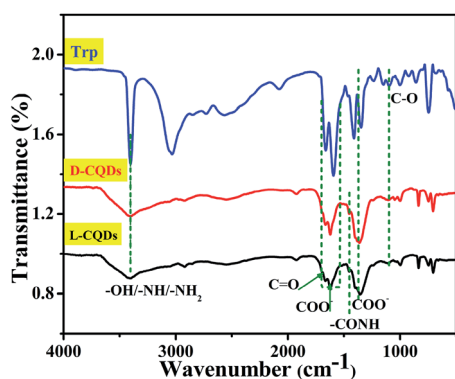
Fig. 4 FT-IR spectra of Trp, L-CQDs and D-CQDs.
