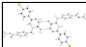
Fig. 2. Dimeric structure formed by hydrogen bonds. Symmetry code: -x + 3, -y + 1, -z + 1
