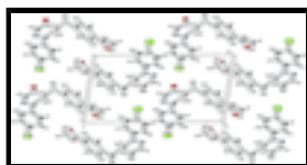
Fig. 4. Packing showing the molecules stacked along [100] direction.
