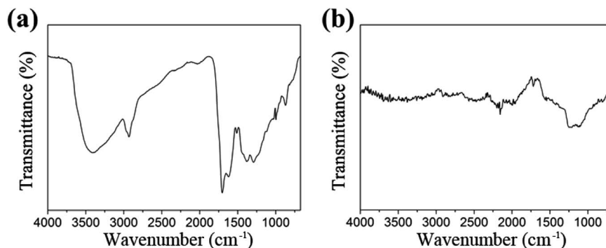
Fig. 4 FTIR spectrum of (a) Mo 2 O 3 @Glc and (b) Mo 2 C@C composites.
