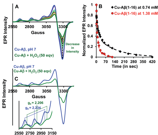
Fig. 3 (A) EPR spectra of Cu-A \beta , blue; Cu-A \beta with 50 eq. H 2 O 2 at different times, green being the final spectrum after 120 minutes; (B) kinetics of the loss of the EPR signal for 50 eq. H 2 O 2 with 0.74 mM Cu-A \beta , black and 1.38 mM Cu-A \beta , red; (C) EPR spectra of Cu-A \beta , blue; Cu-A \beta with 50 eq. H 2 O 2 , green, inset: hyperfine overlay of the data; data are obtained in 100 mM HEPES buffer at pH 7 and 77 K.
