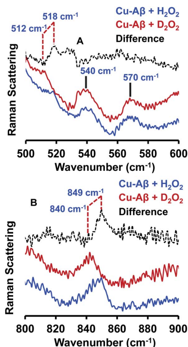
Fig. 4 Resonance Raman spectra of (A) Cu-A \beta + 50 eq. H 2 O 2 , blue and Cu-A \beta + 50 eq. D 2 O 2 in, red; difference spectrum of H 2 O 2 data from D 2 O 2 data, dashed black; lower energy region; (B) Cu-A \beta + 50 eq. H 2 O 2 , blue and Cu-A \beta + 50 eq. D 2 O 2 in, red; difference spectrum of H 2 O 2 data from D 2 O 2 data, dashed black; higher energy region. Data were obtained with an excitation wavelength of 415.4 nm (10 mW at the sample) at 77 K (full spectra in Fig. S5†).
