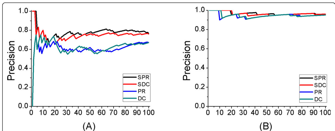
Figure 2 Comparison of results for PageRank and degree centrality when being applied on the original protein interaction network (PIN) and tissue specific network (TSN). The x axis represents the number of identified disease-related genes. The y axis represents the predicted precision of each result. (A) Results on colon cancer. (B) Results on leukemia.
