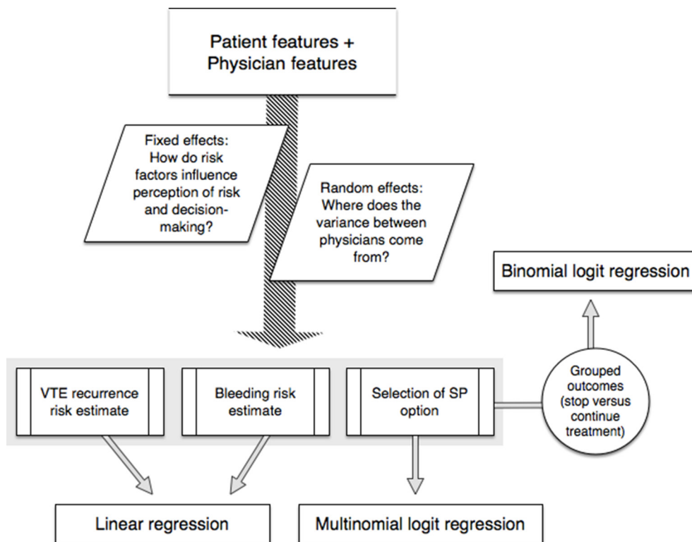
Figure 4 Analysis flowchart.
