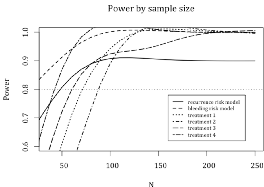
Figure 2 Power by sample size.
