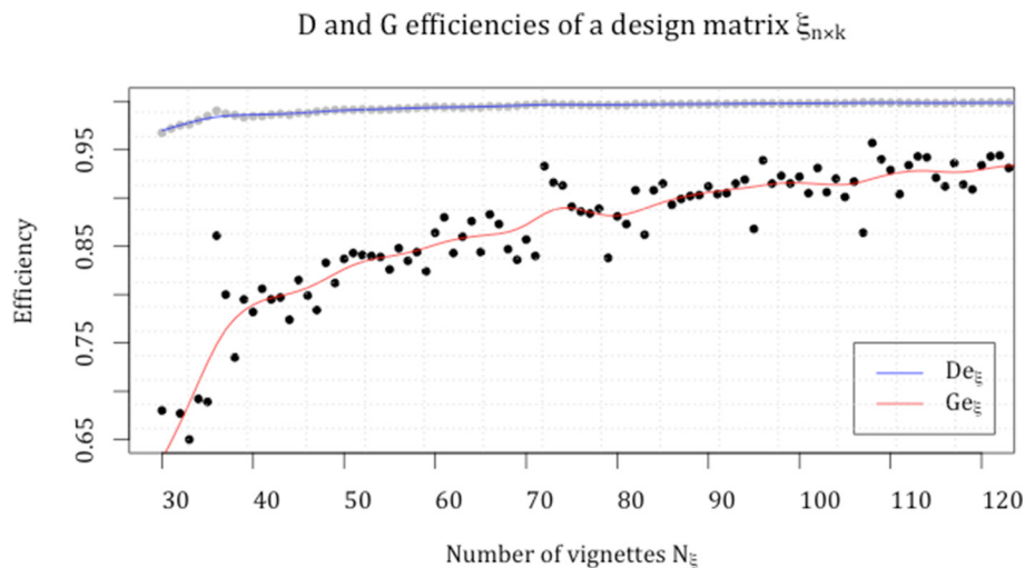
Figure 1 D and G efficiencies of design matrix \xi .
