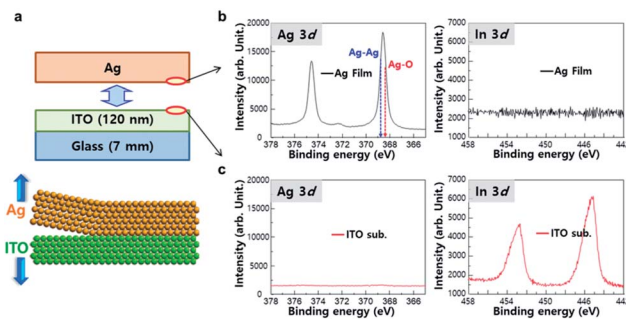
Fig. 2 Interfacial reactions between Ag layer and ITO substrate on peel-off process. (a) Schematic drawing of Ag film peeled-off from ITO substrate. (b) Ag 3d and In 3d SRPES spectra of the surface of peeled-off Ag film. (c) Ag 3d and In 3d SRPES spectra at the surface of peeled-off ITO layer.
