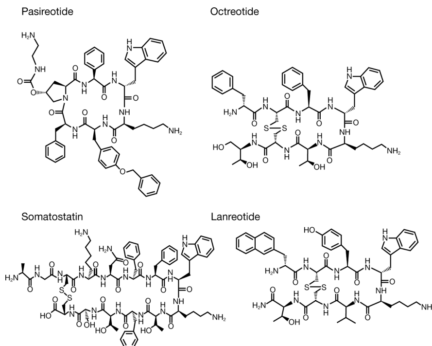
Figure 1 Chemical structures of pasireotide, somatostatin (SRIF-14) and other somatostatin analogs.
