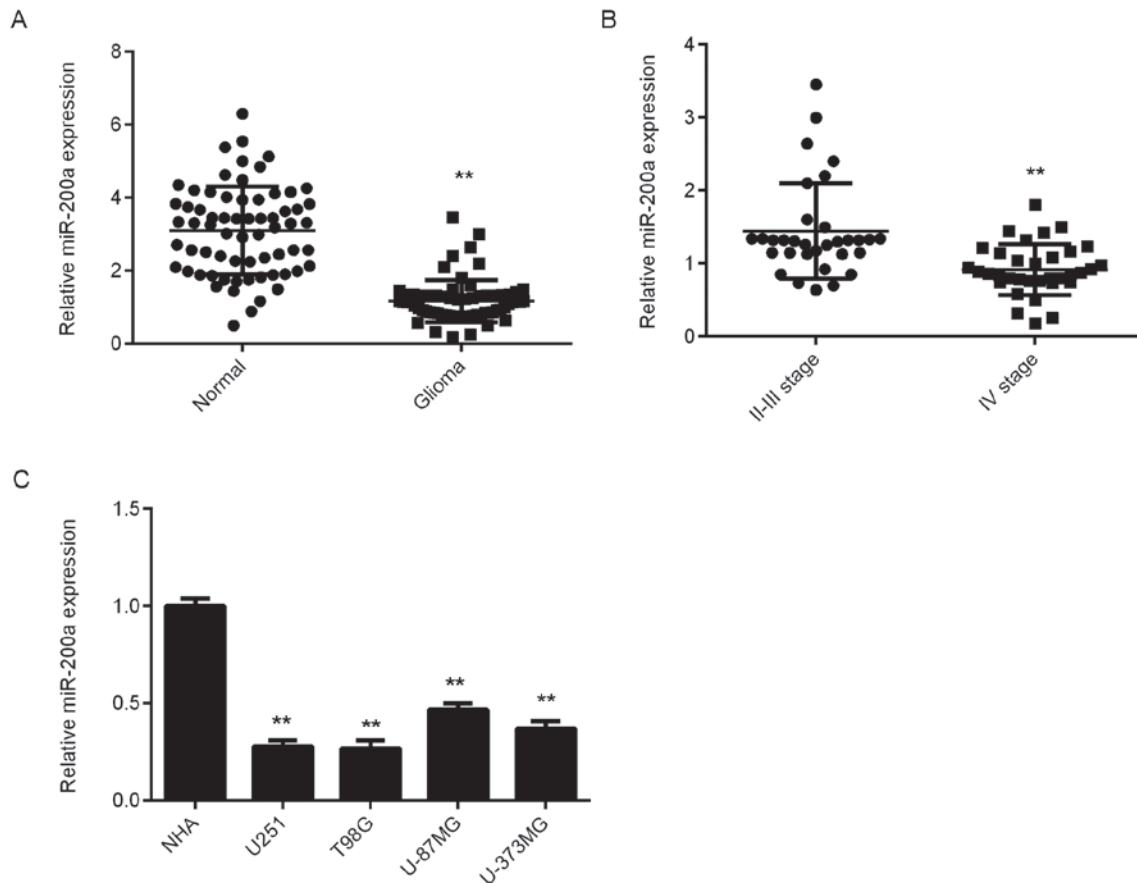
Figure 1. (A) RT-qPCR data indicated that the expression of miR-200a was lower in glioma tissues compared with those in normal brain tissues. ** P < 0.01 vs. normal tissues. (B) RT-qPCR data indicated that the levels of miR-200a were lower in glioma tissues at stage IV compared with those at stages II-III. ** P < 0.01 vs. II-III stage. (C) RT-qPCR demonstrated that miR-200a was significantly downregulated in glioma cell lines compared with NHA cells. ** P < 0.01 vs. NHA. RT-qPCR, reverse transcription-quantitative polymerase chain reaction; miR, microRNA; NHA, normal human astrocyte.
