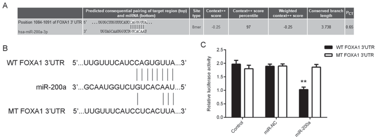
Figure 3. (A) TargetScan software data indicated that the 3'UTR of FOXA1 mRNA contained the binding sequences of miR-200a. (B) The WT FOXA1-3'UTR and the MT FOXA1 3'UTR luciferase reporter plasmids were generated. (C) Dual luciferase reporter gene assay was then conducted in T98G cells. ** P < 0.01 vs. control. UTR, untranslated region; FOXA1, forkhead box A1; miR, microRNA; WT, wild type; MT, mutant type; P CT , the probability of conserved targeting.
