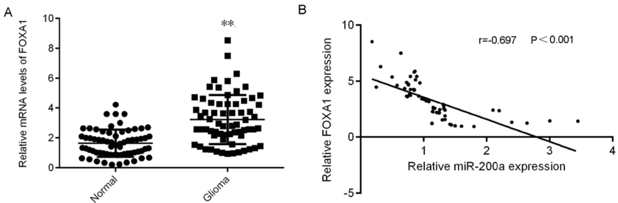
Figure 4. (A) Reverse transcription-quantitative polymerase chain reaction data demonstrated that FOXA1 was significantly upregulated in glioma tissues compared with normal brain tissues. (B) A negative correlation was observed between FOXA1 and miR-200a expression in glioma tissues. ** P < 0.01 vs. normal. FOXA1, forkhead box A1; miR, microRNA.
