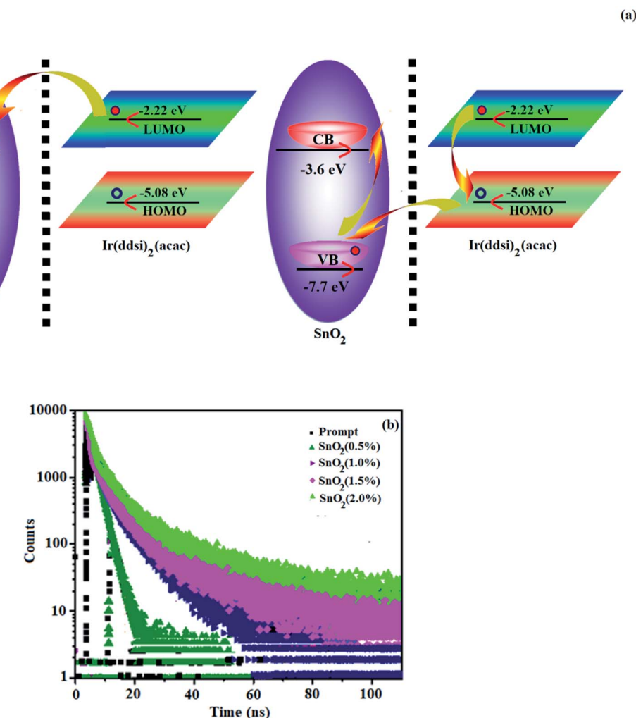
Fig. 7 (a) Exciton dissociation SnO 2 :Ir(dds) 2 (acac) interface and non-radiative energy transfer from Ir(dds) 2 (acac) to SnO 2 NPs and (b) lifetime decay of devices.
