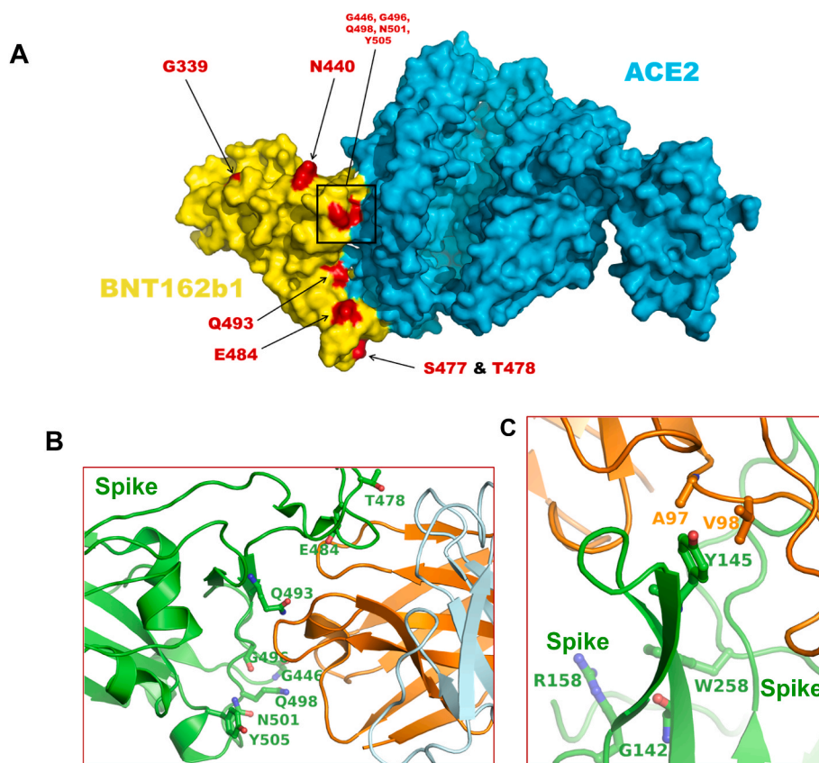
Fig. 2. Distribution of amino acid residue position at Spike/ACE2 or Spike/antibody interface. Panel A shows the distribution of amino acid residues mutated in the Omicron variant in the complex formed between S-RBD encoded by BNT162b1 and ACE2. This figure has been generated by PDB entry 7L7F. Panel B shows the position of residues at the interface of S-RBD and antibody IGHV3-53, where the mutations in Omicron variant have been identified. The S protein is rendered in green ribbons, whereas the antibody is rendered in orange and light-blue ribbons. The amino acid residues representing the mutation sites in the Omicron variant are rendered as balls and sticks. Panel C shows the interaction Y145 of S protein with antibody (1–87) residues A97 and V98. A deletion mutation (as seen in Omicron variant) will abrogate these interactions. This figure also shows some residue positions in S protein where the mutations in Delta and Delta Plus variants are present. Figures for Panel D and E were generated from PDB entries 7JMP and 7L2D, respectively. In both panels, the atoms of S protein residues are colored as green – carbons, blue – nitrogens, and red – oxygens. Atoms of antibodies are colored as orange – carbons, blue – nitrogens, and red – oxygens.
