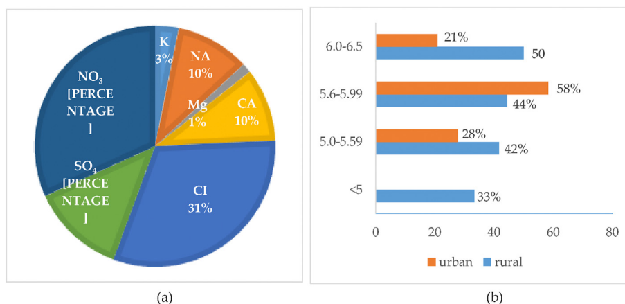
Figure 3. Overall total percentage (%) of ions compositions (a); pH frequency (%) of rainwater (b).
