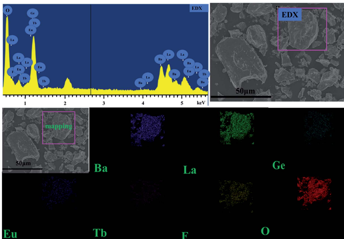
Fig. 3 (Top right) SEM image of BLGeOF:0.15Tb 3+ , 0.15Eu 3+ phosphor (Top left) EDX spectra of BLGeOF:0.15Tb 3+ , 0.15Eu 3+ phosphors (Bottom) elemental distribution of BLGeOF:0.15Tb 3+ , 0.15Eu 3+ phosphors.
