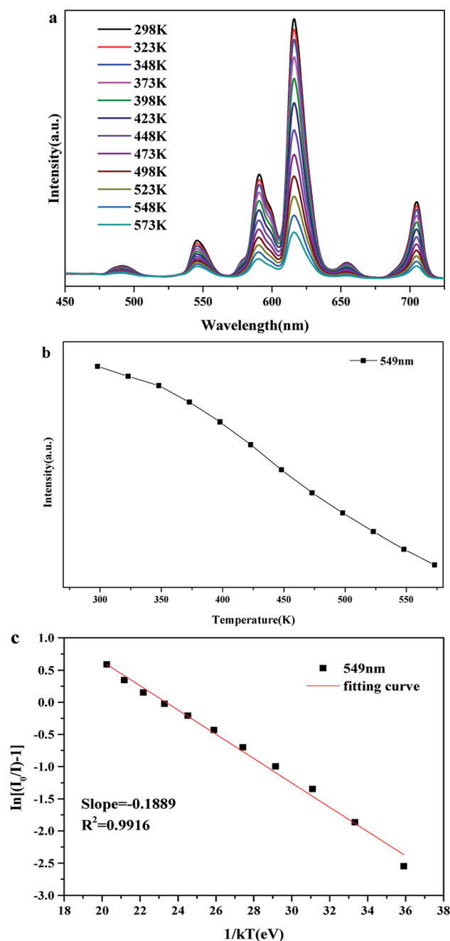
Fig. 12 (a) The luminescence spectra of \text{BLGOF}:0.15\text{Tb}^{3+}, 0.24\text{Eu}^{3+} at different temperatures (b) the intensity changes of \text{BLGOF}:0.15\text{Tb}^{3+}, 0.24\text{Eu}^{3+} phosphors 549 nm emission peak at different temperatures (c) \ln(I_0/I - 1) versus 1/kT for the \text{BLGOF}:0.15\text{Tb}^{3+}, 0.24\text{Eu}^{3+} .
