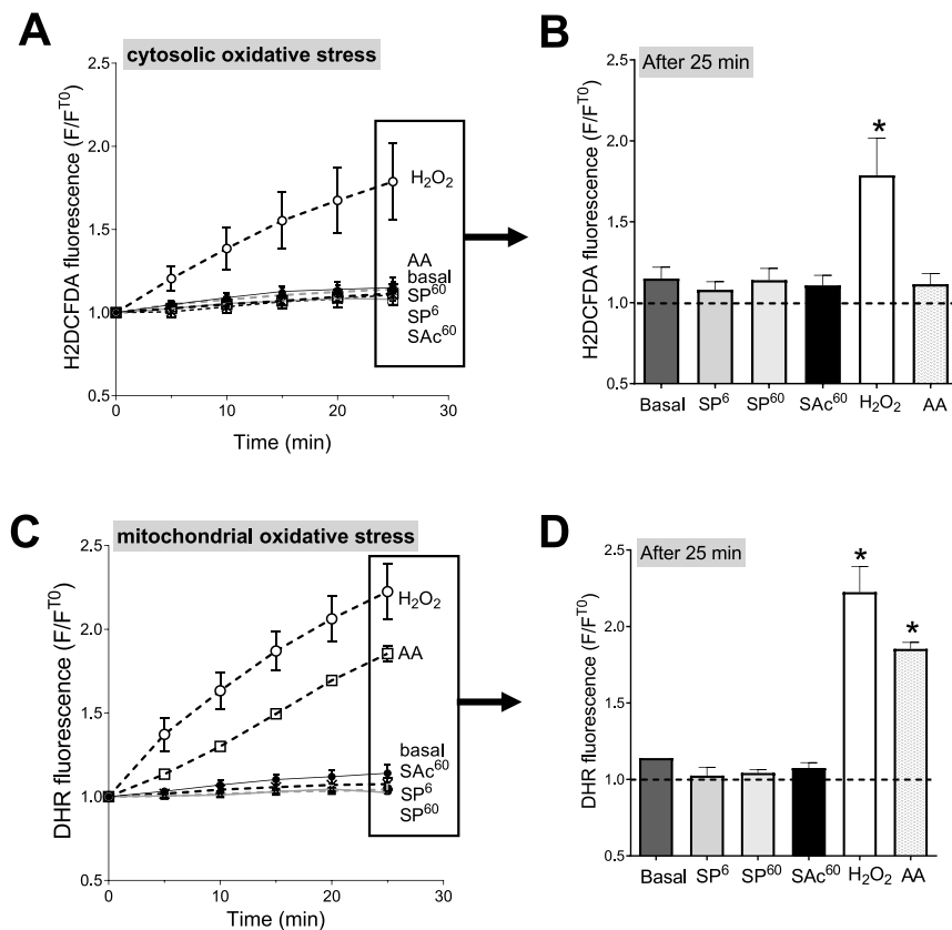
Fig. 4. \text{H}_2\text{O}_2 and antimycin A-induced oxidative stress in cardiomyocytes. Cardiomyocytes were loaded with fluorogenic dyes sensitive to ROS production. \text{H}_2\text{DCFDA} dye (A, B) probes oxidative stress within the cytosol. Dihydrorhodamine 123 (DHR 123 ) dye (C, D) probes oxidative stress within the mitochondria. Fluorescence was measured every 5 min and was normalized by baseline fluorescence ( T_0 ) (A, C). In control cells (basal), the fluorescence increases modestly during the 25 min-period. Some myocytes were incubated for 1 h with either 6 \mu\text{M} of sinapine ( \text{SP}^6 ), 60 \mu\text{M} of sinapine ( \text{SP}^{60} ) or 60 \mu\text{M} of sinapic acid ( \text{SAC}^{60} ) prior to measurement. Some cells were stimulated with 0.1 mM \text{H}_2\text{O}_2 or with a mitochondrial electron transport chain complex III blocker, antimycin A (AA, 10 \mu\text{M} ) to force mitochondria to produce ROS. The fluorescence in each condition was compared with control cells (basal). (B, D) Representative average fluorescence after 25 min from graphs A and C. ( n = 4 animals) (A, B) Linear mixed model effect: Time: p < 0.001 , Group: p = 0.0139 , Time-Group: p < 0.001 . (C, D) Linear mixed model effect: Time: p < 0.001 , Group: p < 0.001 , Time-Group: p < 0.001 . *, p < 0.05 , **, p < 0.01 .
