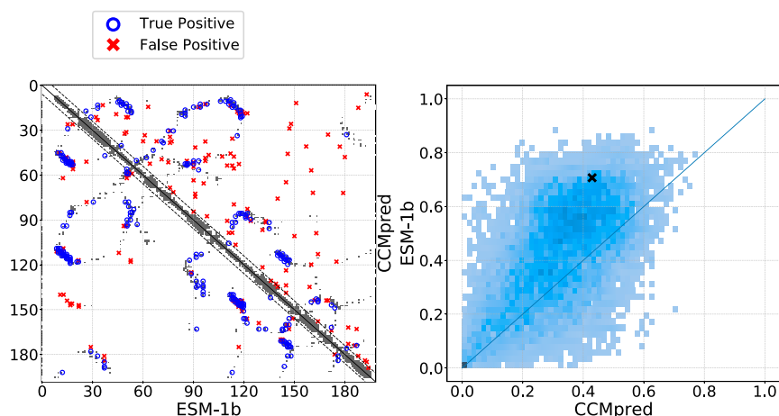
Fig. 5. Residue-residue contacts (linear projections). (Left) Top-L predictions for fold level held-out example d1n3ya_, with vWA-like fold. True positives in blue, false positives in red, superimposed on ground truth contact map in gray. ESM-1b Transformer projections below the diagonal, CCMpred predictions above the diagonal. (Right) Precision distribution (top-L long-range) comparing ESM-1b projections with CCMpred across all domains in the five test partitions with structural holdout at the fold level. Visualized domain marked by \times .
