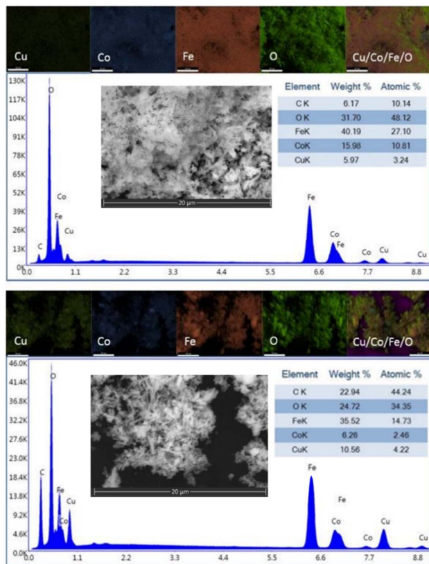
Fig. 2 SEM/EDX and elemental mapping for \text{Cu}_x\text{Co}_{1-x}\text{Fe}_2\text{O}_4 ( x = 0.2 (top panel) and 0.6 (bottom panel)) NFs. In the elemental analysis graph, the X-axis represents energy (eV) and the Y-axis represents intensity ( k ).
