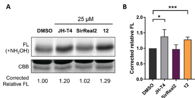
Fig. 8 Investigation of the inhibition of Sirt2 defatty-acylation activity in cells. (A) Detection of KRas4a fatty acylation levels after treatment with Sirt2 inhibitors (25 \mu\text{M} ) or DMSO ( n = 4 ). FL: Fluorescence, CBB: Coomassie blue. (B) Quantified relative fluorescence signals of the Sirt2 inhibitors and the DMSO control. Error bars represent mean \pm SD. Statistical evaluation was performed using a Student's t test. * p < 0.05 , *** p < 0.001 .
