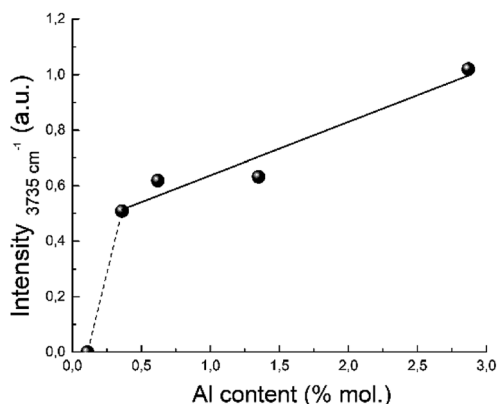
Fig. 13 Correlation between the 3735 cm -1 IR band intensity and the aluminum content.
