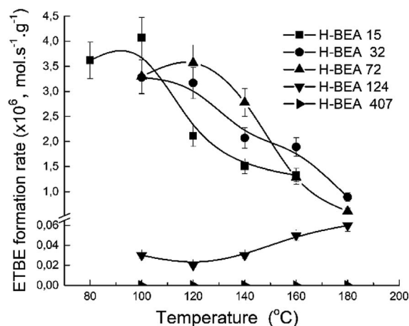
Fig. 11 Temperature dependence of apparent ETBE formation rate for zeolites H-BEA.
