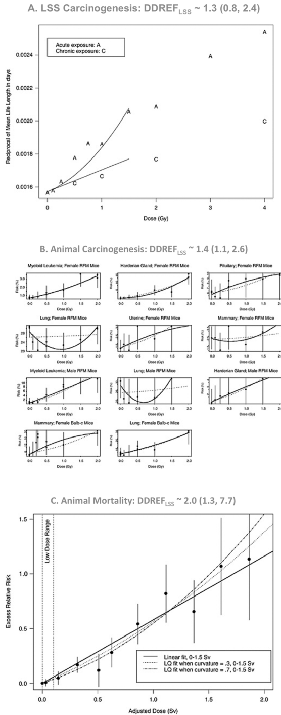
Fig 3. BEIR VII DDREF_{LSS} estimates from 3 data sources. Reprinted with permission from figures 10–2, 10B–2, and 10B–3 of “Health risks from exposure to low levels of ionizing radiation: BEIR VII phase 2” [2]. Linear-quadratic models used for DDREF_{LSS} evaluation fit to three data sources, (A) excess risk of carcinogenesis in atomic bomb survivors, (B) risk of tumor development in various animal studies, and (C) inverse mean lifespan in two animal studies. All panels show dose (x-axis) vs. various measurements of risk (y-axis). Best-fit linear-quadratic models are shown for each model. The LSS carcinogenesis data shows best-fit models with various curvatures. Animal carcinogenesis data shows best-fit models for each panel individually (solid black lines) and the consensus curvature across all panels (dashed lines). The animal mortality data shows the single best-fit model with both acute (linear-quadratic) and protracted (linear) projections. Only animal mortality data included both acute, “A”, and protracted, “C”, exposures. Above each
