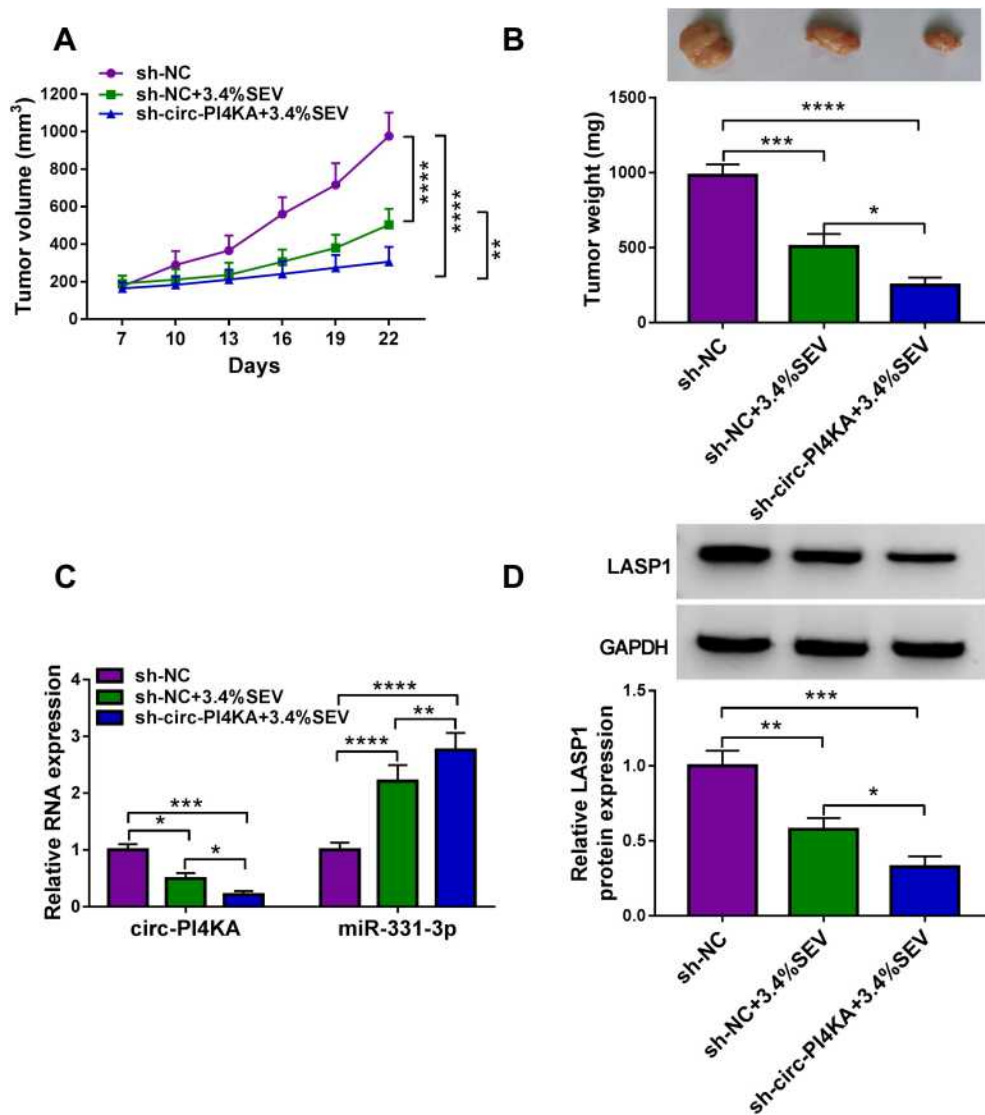
Figure 9 Circ-PI4KA silencing facilitated the effects of SEV treatment on tumor growth in vivo. (A and B) The effects between SEV treatment and circ-PI4KA depletion on tumor volume and weight were unveiled in vivo. (C) The impacts between SEV treatment and circ-PI4KA repression on the expression of circ-PI4KA and miR-331-3p were demonstrated by qRT-PCR in vivo. (D) Western blot was conducted to disclose the influence of circ-PI4KA knockdown on LASP1 protein expression under SEV exposure in vivo. * P < 0.05 , ** P < 0.01 , *** P < 0.001 and **** P < 0.0001 . Circular RNA phosphatidylinositol 4-kinase alpha (circ-PI4KA); sevoflurane (SEV); LIM and SH3 protein 1 (LASP1); quantitative real-time polymerase chain reaction (qRT-PCR).
