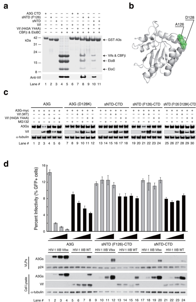
Figure 4. Functional assays of sNTD. (a) E. coli co-expression and GST-pull down assay of sNTD and the Vif, CBFβ, elongin B, elongin C complex (VCBC complex). Samples are GST-fused A3G CTD (lanes 6 and 7), GST-fused sNTD(F126) (lanes 8 and 9) or GST-fused sNTD (lanes 10 and 11) expressed together with untagged CBF-β, elonginBC and wild type HIV-1 Vif or Vif(H43A Y44A). Lanes 1–5 show reference bands for the expressed protein. (b) Locations of D128 and A126 (displayed in green) in the sNTD structure. (c) Vif-mediated degradation assay using wildtype A3G (A3G) (lanes 1–6), A3G with D128K substitution [A3G(D128K)] (lanes 7–12), sNTD fused with wild type CTD (sNTD-CTD) (lanes 13–18), sNTD with A126F substitution fused with wild type CTD [sNTD(F126)-CTD] (lanes 19–24) and sNTD with A126F and D128K double-substitutions fused with wild type CTD [sNTD(F126 D128K)-CTD] (lanes 25–30). Alpha-isoform of tubulin ( \alpha -
