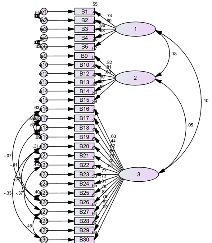
Figure 2 Standardised three-factor structural equation model diagram.
