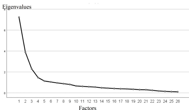
Figure 1 The screen plot.
