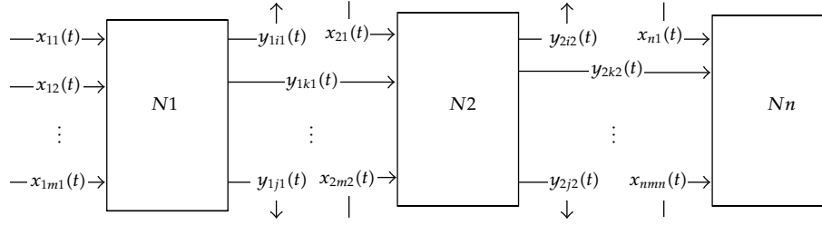
FIGURE 2: Tandem network.
