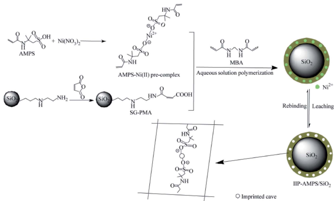
Fig. 10 Synthetic procedure for IIP-AMPS/ \text{SiO}_2 (this figure has been adapted/reproduced from ref. 119 with permission from Chinese Chemical Society, Institute of Chemistry, Chinese Academy of Sciences and Springer-Verlag GmbH Germany, part of Springer Nature, copyright 2018).
